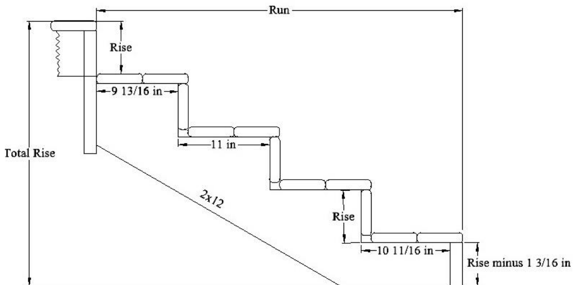
Figure C1 Stair stringer
