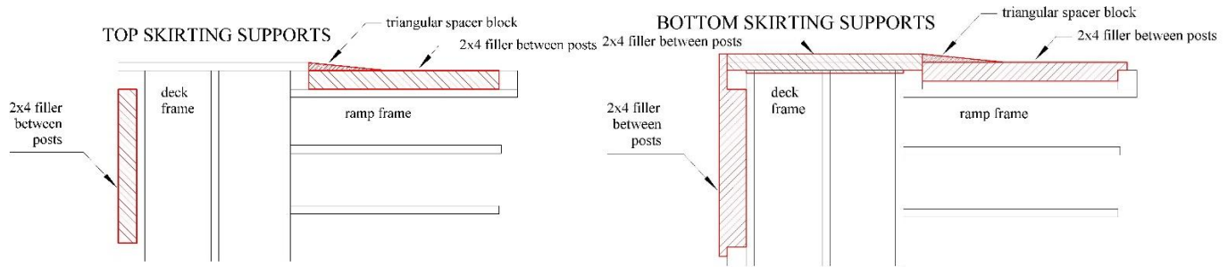
Figure D2. 2x4 filler and triangular spacer block provides a smooth surface for the skirting
