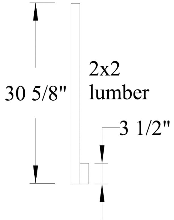
Figure E5 Handrail toe board spacer tool.
