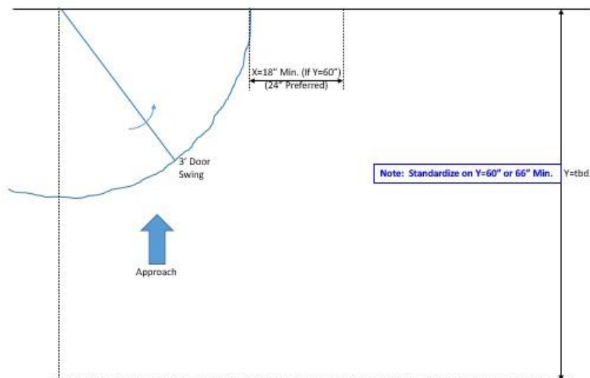
Figure 10 – Maneuvering Clearance at Doors
